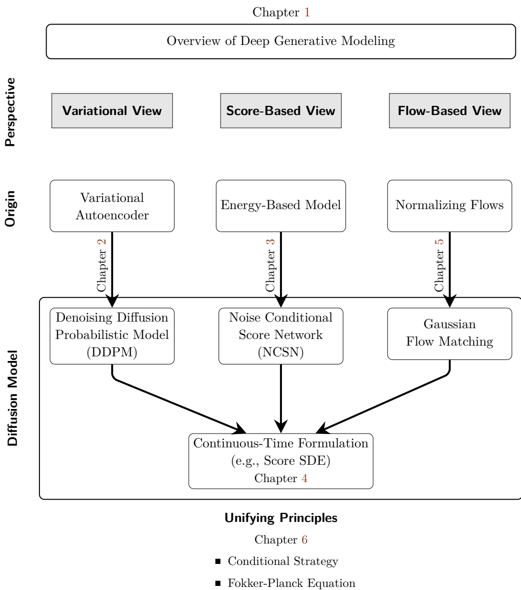
Figure 3: Part B. Unifying and Principled Perspectives on Diffusion Models. This diagram visually connects classical generative modeling approaches—Variational Autoencoders, Energy-Based Models, and Normalizing Flows—with their corresponding diffusion model formulations. Each vertical path illustrates a conceptual lineage, culminating in the continuous-time framework. The three views (Variational, Score-Based, and Flow-Based) offer distinct yet mathematically equivalent interpretations.
